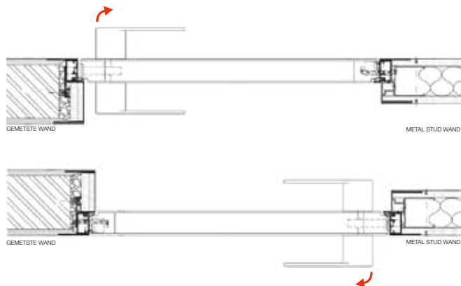
INSTALLATIE TREKKEND EU LINKS
